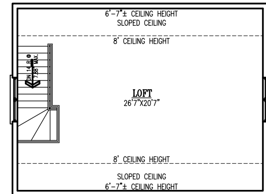
LOFT FLOOR PLAN 591 SQ. FT.
