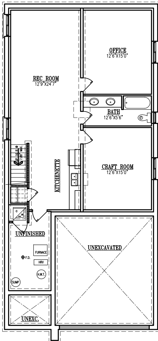
OPT. FINISHED BASEMENT 956 SQ. FT. FINISHED
