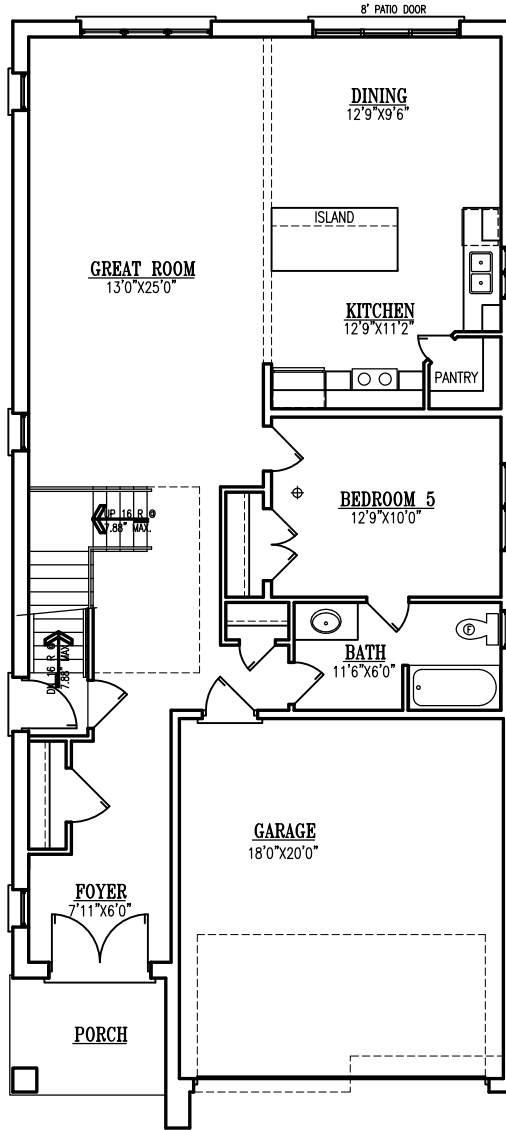
MAIN FLOOR PLAN 1219 SQ. FT. (2762 SQ. FT. TOTAL)
