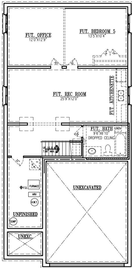
OPT. FINISHED BASEMENT 850 SQ. FT. FUTURE FINISHED
